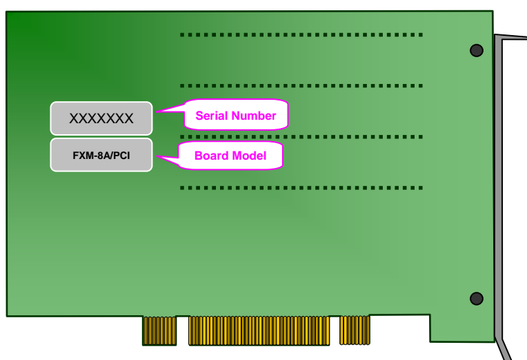
Figure 2-2 FXM-8A/PCI (Rear View)
